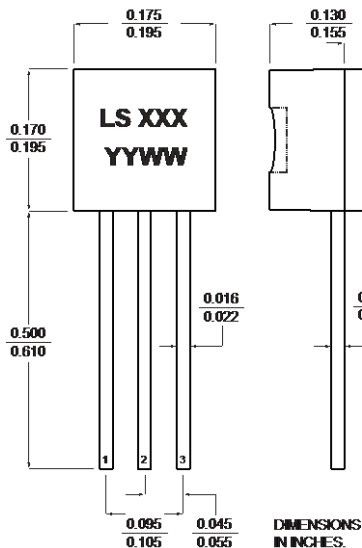
TO-92 3 Lead
