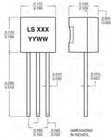
TO-92
