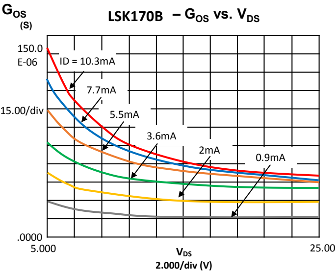
Output Conductance
