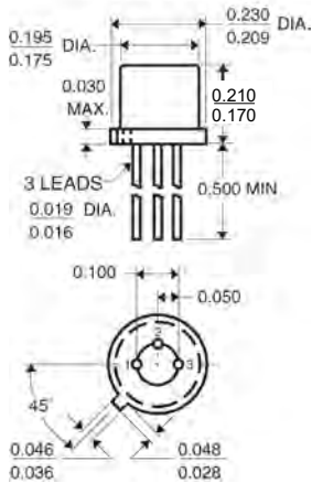
TO-18
