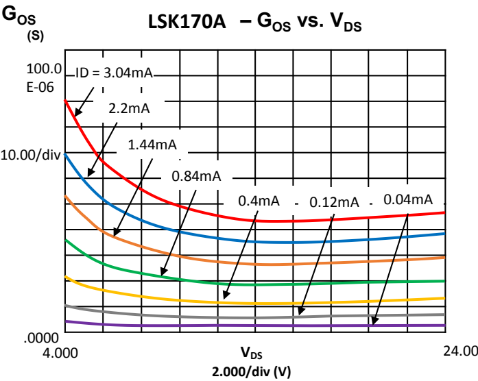
Output Conductance
