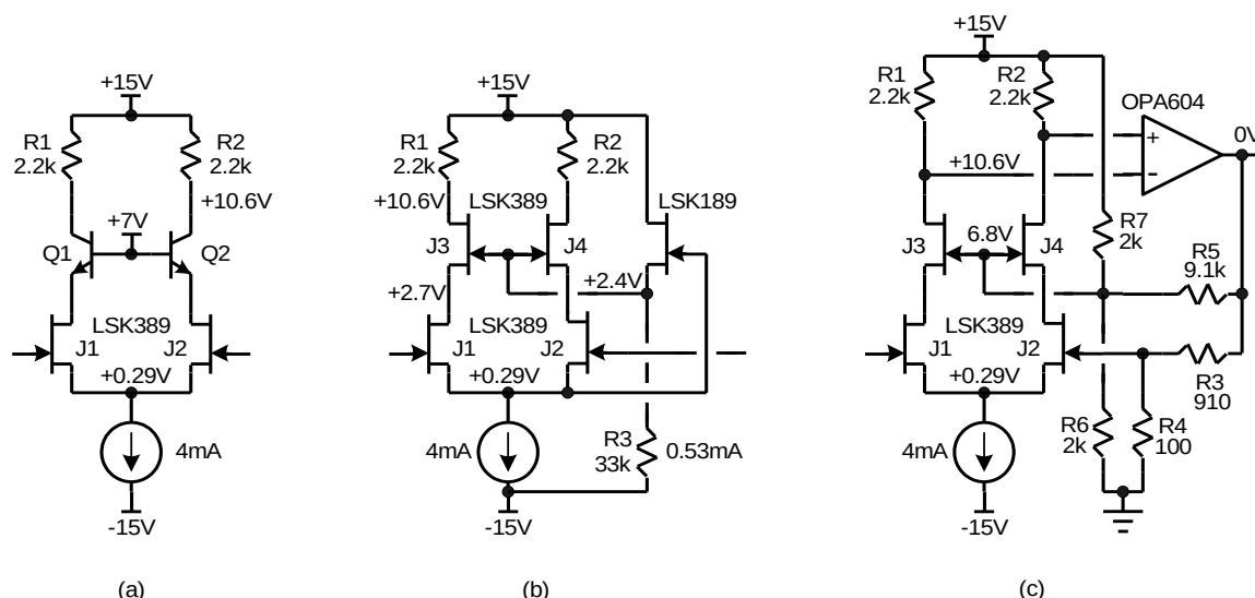
Figure 5: Cascoded differential amplifiers
