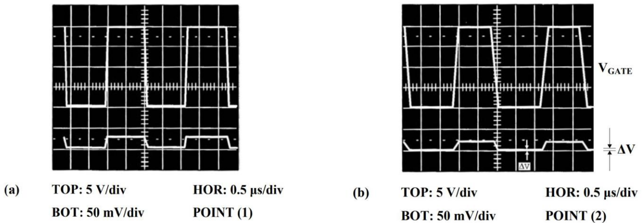
Figure 10. Waveforms for Points (1) and (2) of Figure 9
