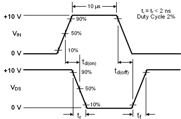
TIMING WAVEFORMS
